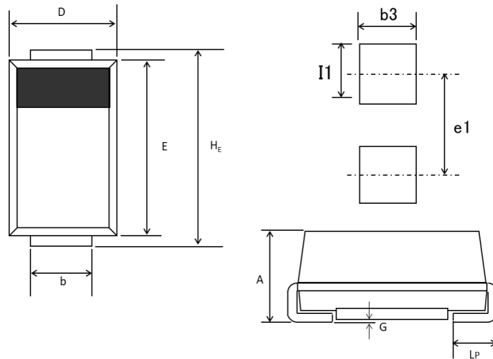
DO-214AC(SMA), (FMDS)
