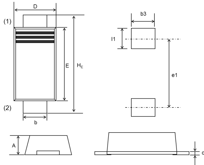
SOD-123FL (FMDU)
