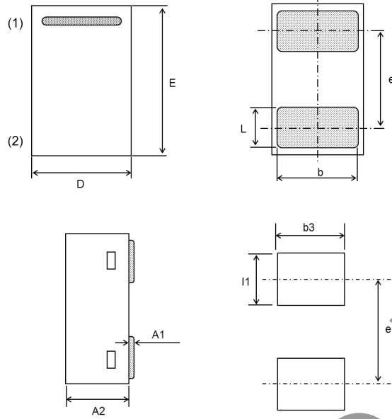
DFN1608-2, (KMD2)
