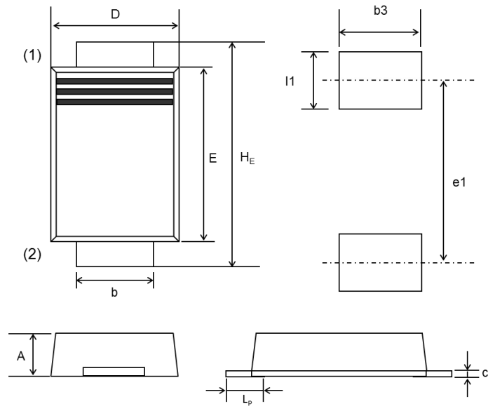
SOD-128, (FMD™)
