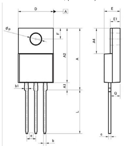
TO-220FN, (TO-220FN)
