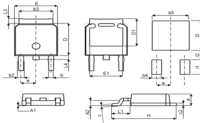
TO-252, (TO-252)
