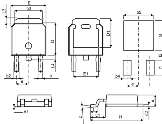
TO-252, (TO-252GE)
