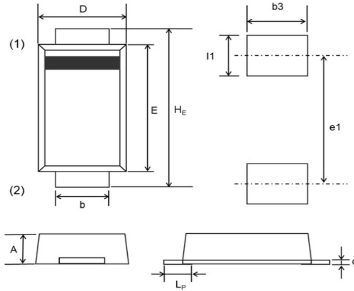
SOD-128
