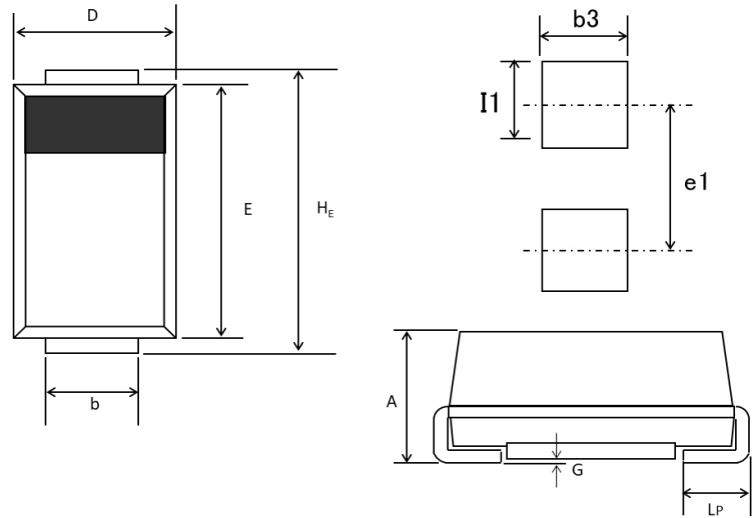
DO-214AC(SMA), (FVDS)
