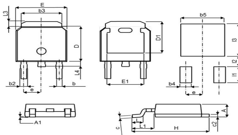
TO-252, (TO-252GE)
