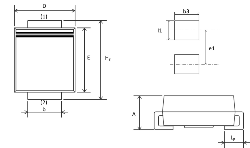
DO-214AA (SMB), (SMBP)
