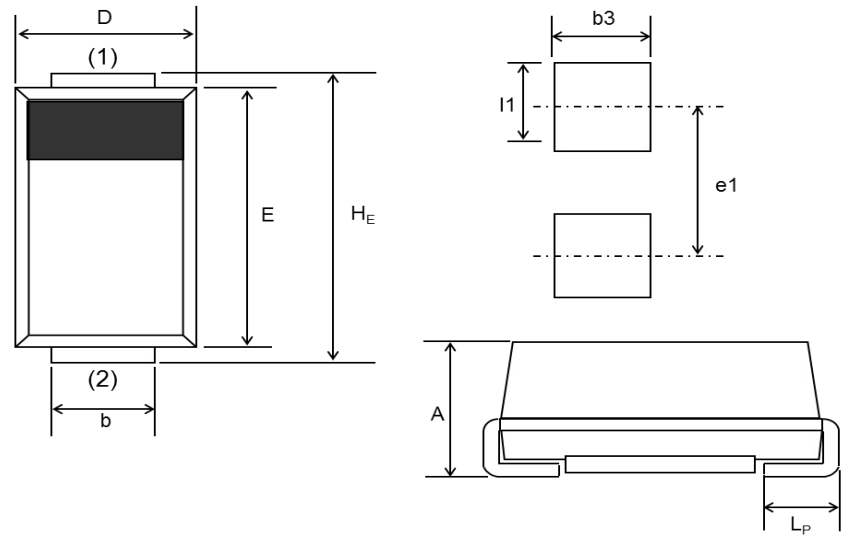
DO-214AC(SMA), (PMDS)
