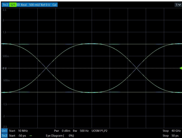
Data Rate > 20 Gbps Eye Diagram (Bare board)
