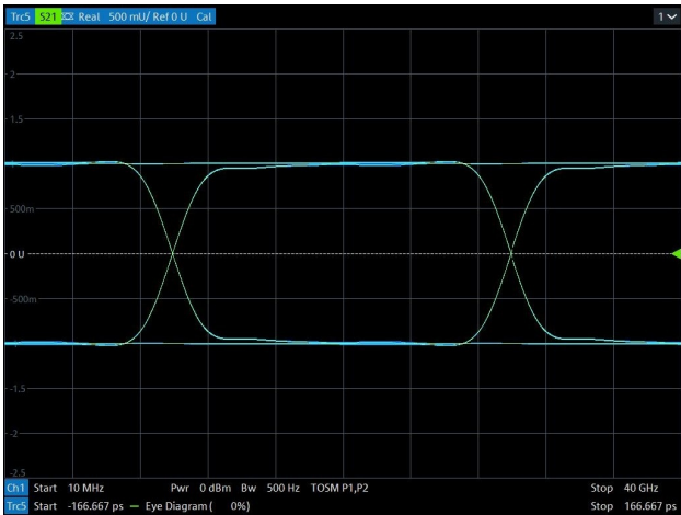
Data Rate > 6 Gbps Eye Diagram (with RES3V3BAED)
