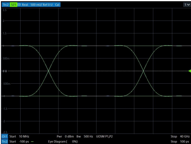
Data Rate > 10 Gbps Eye Diagram (Bare board)
