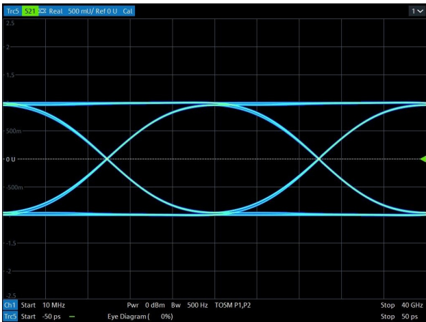
Data Rate > 20 Gbps Eye Diagram (with RES3V3BAED)
