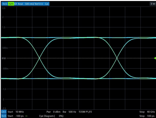
Data Rate > 10 Gbps Eye Diagram (with RES3V3BAED)
