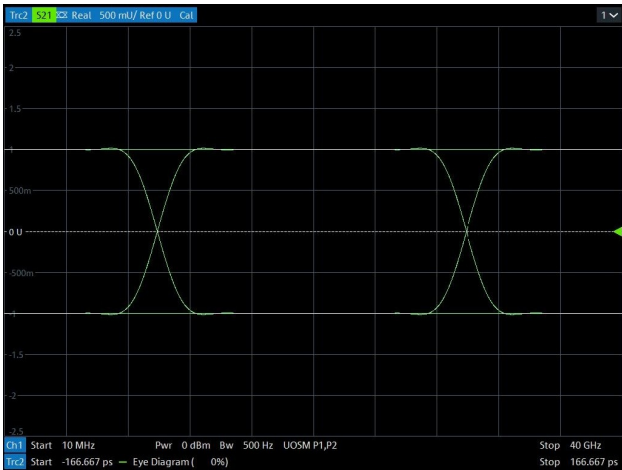
Data Rate > 6 Gbps Eye Diagram (Bare board)
