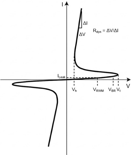
I-V characteristics for a bidirectional ESD protection diode
