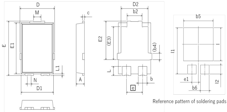
TO-277A
