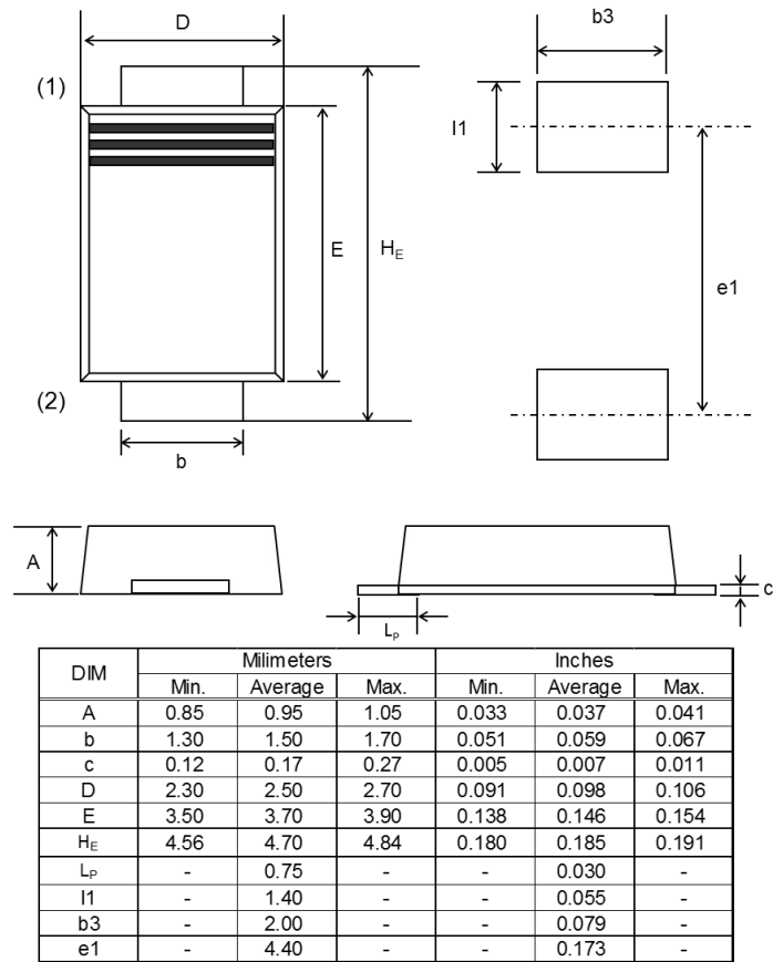
SOD-128, (PMDTM)
