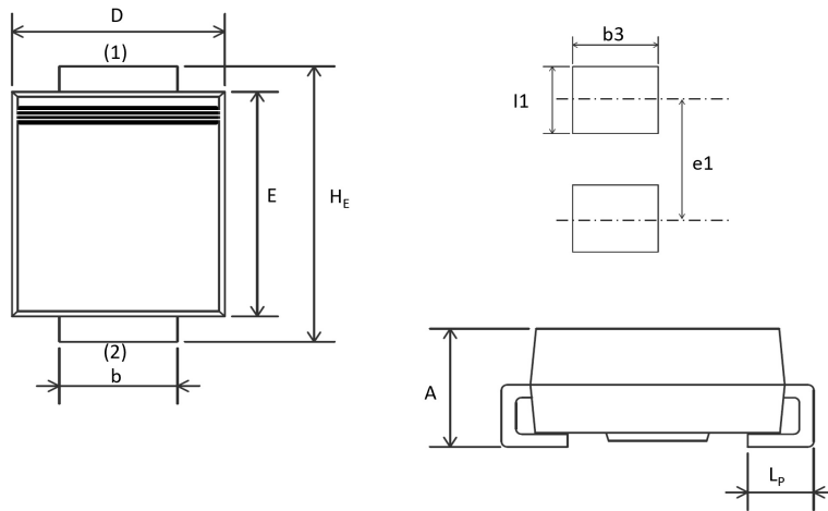
DO-214AA (SMB)
