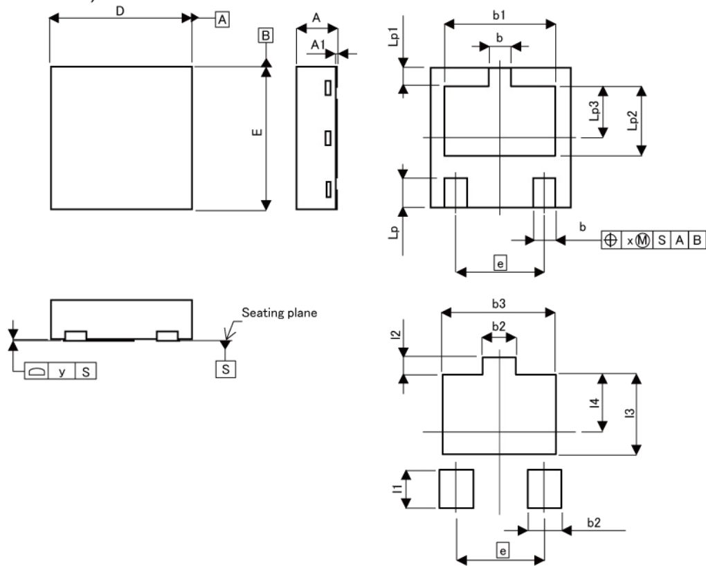
DFN2020-3S ( HUML2020L3 )
