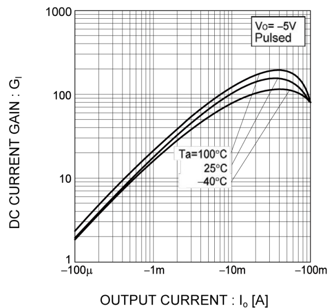
Fig.4 DC current gain vs. output current
