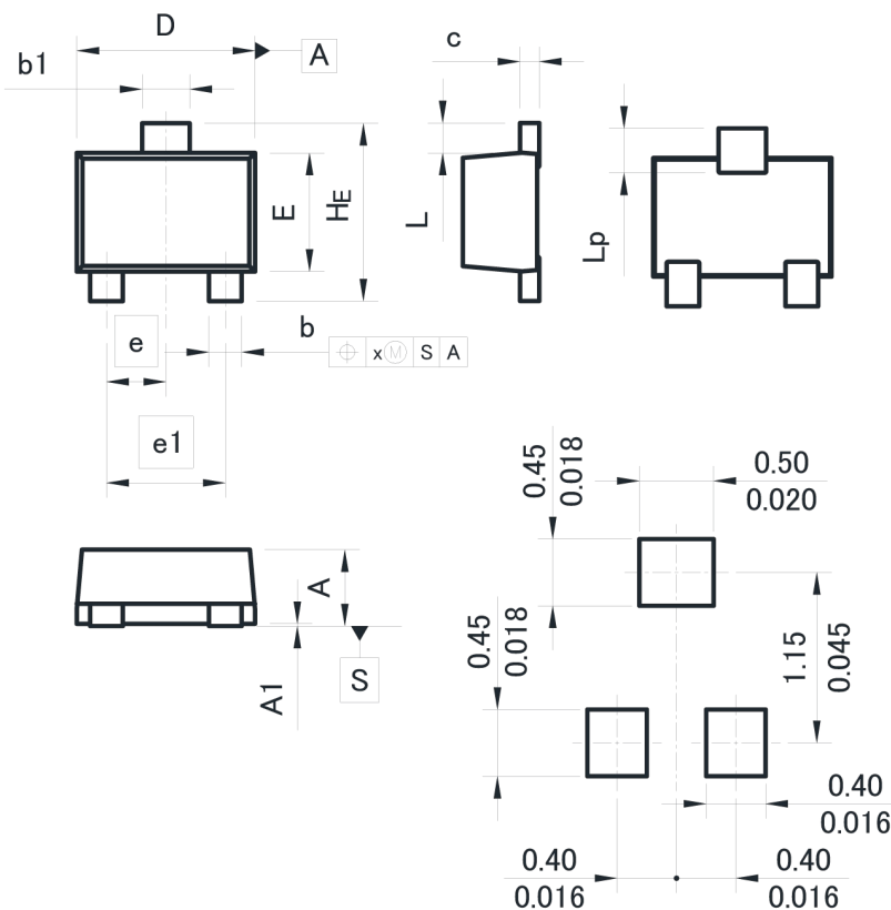
Soldering footprint Unit: ( \frac{\text{mm}}{\text{inches}} )
