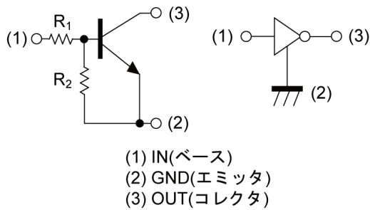
DTC124XM
