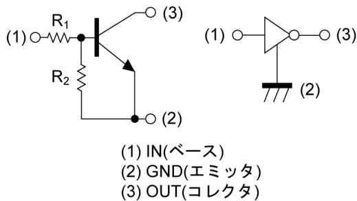
DTC124XM
