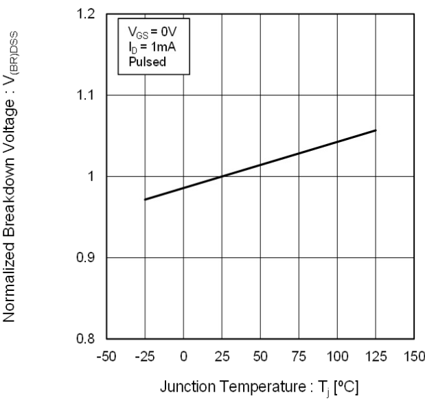
Fig.7 Normalized Breakdown Voltage vs. Junction Temperature
