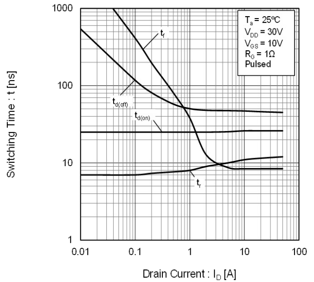
Fig.18 Switching Characteristics
