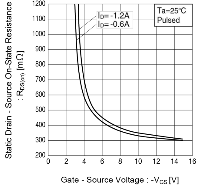
Fig.5 Static Drain - Source On - State Resistance vs. Gate Source Voltage
