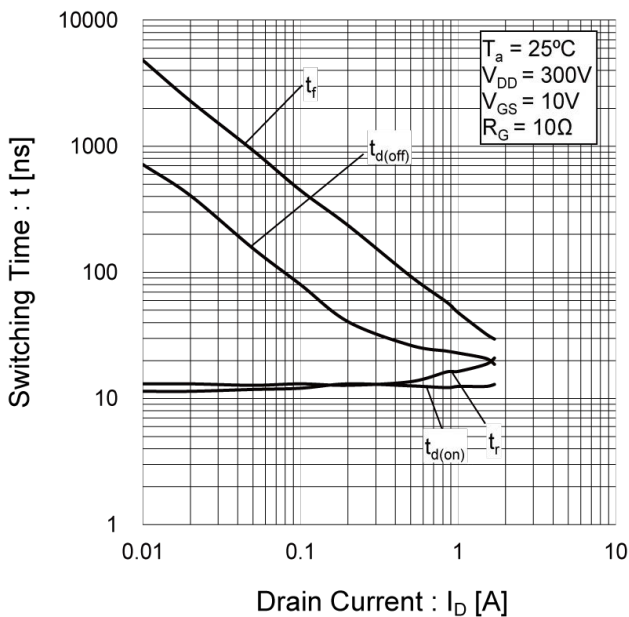
Fig.15 Switching Characteristics
