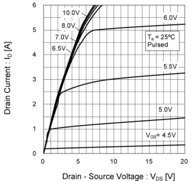
Fig.8 Output Characteristics(II)
