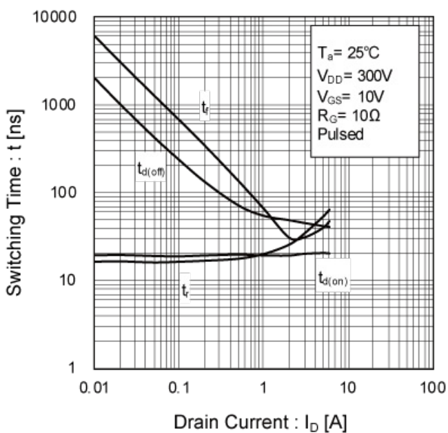
Fig.15 Switching Times
