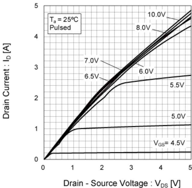
Fig.7 Output Characteristics(I)
