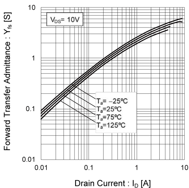
Fig.12 Forward Transfer Admittance vs. Drain Current
