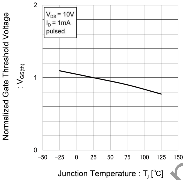
Fig.9 Normalized Gate Threshold Voltage vs Junction Temperature
