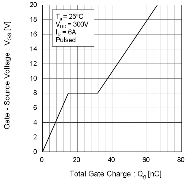
Fig.16 Gate Charge
