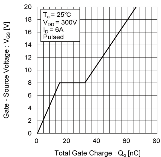
Fig.16 Gate Charge
