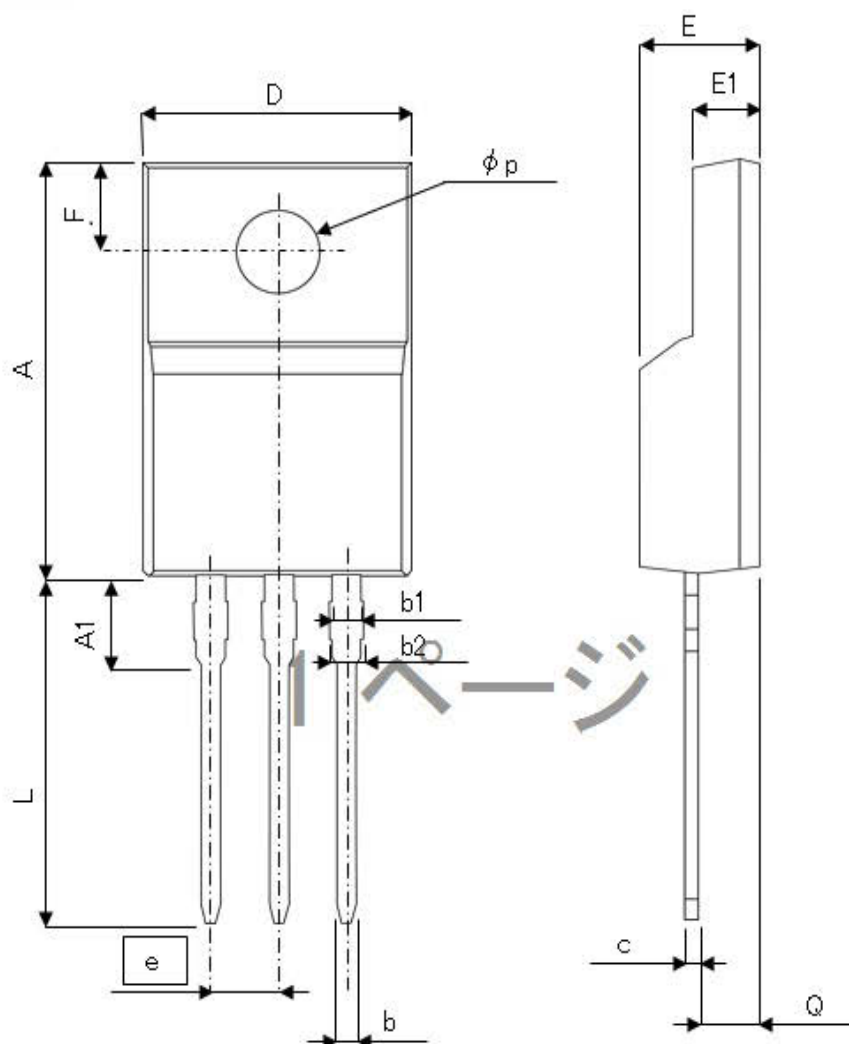
TO-220FM
