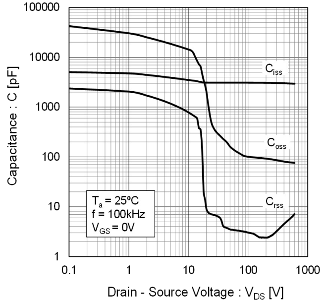
Fig.14 Capacitances
