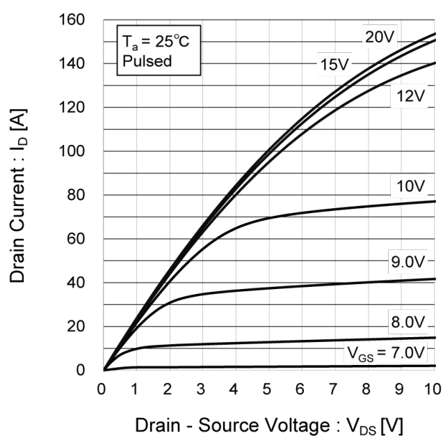
Fig.8 Output Characteristics(II)
