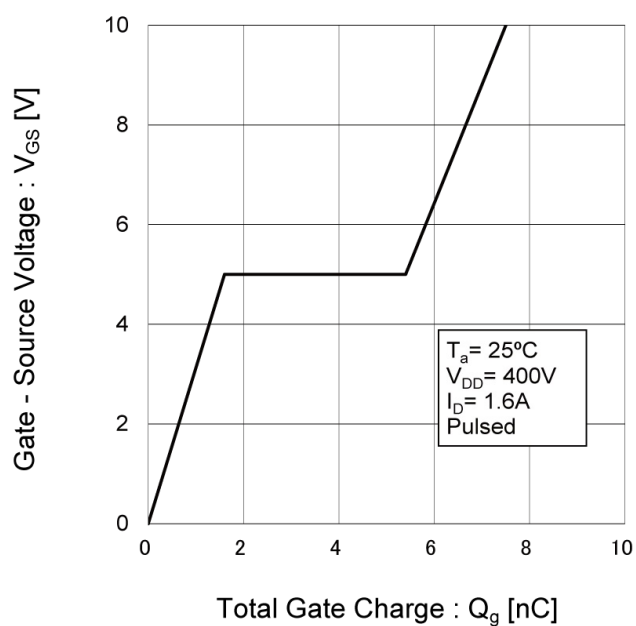
Fig.16 Gate Charge
