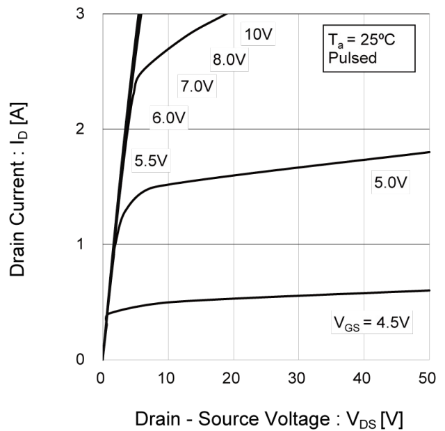
Fig.8 Output Characteristics(II)
