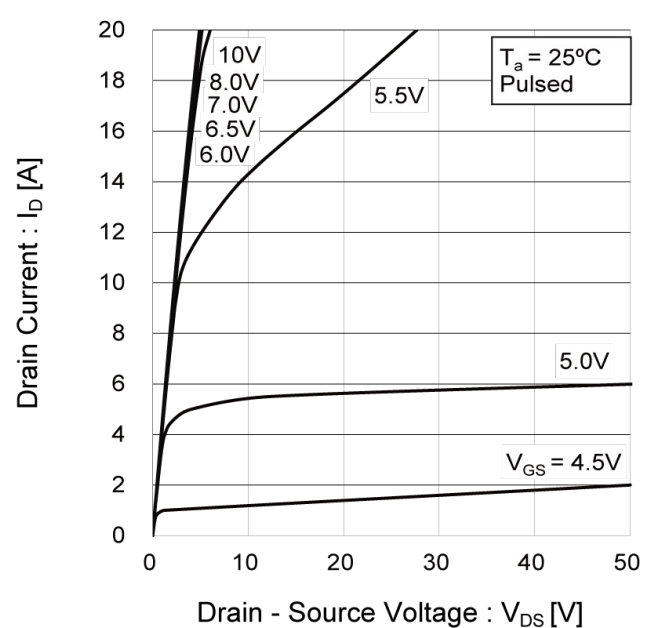
Fig.8 Output Characteristics(II)
