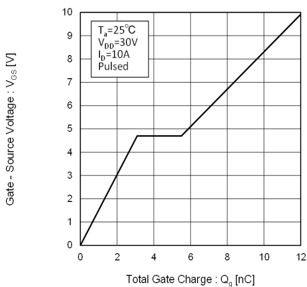
Fig.19 Dynamic Input Characteristics
