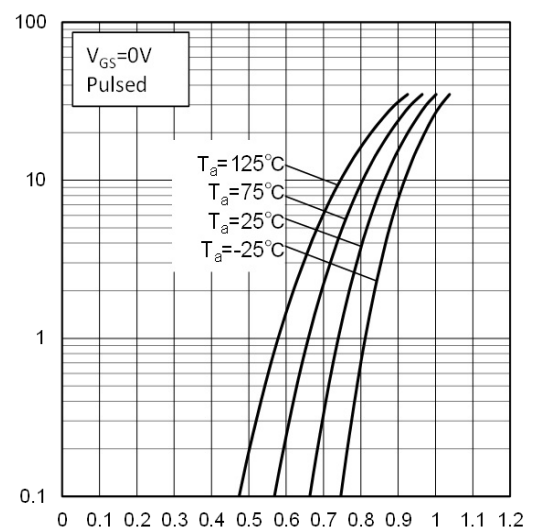
Fig.20 Source Current vs. Source Drain Voltage
