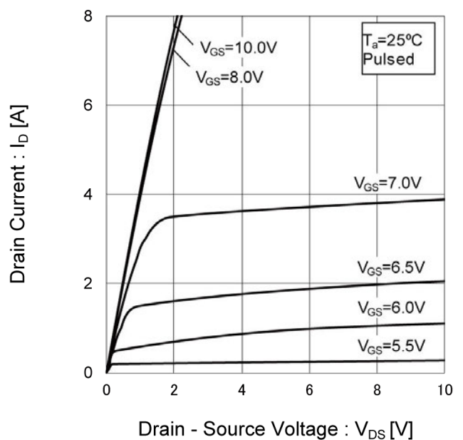
Fig.8 Output Characteristics(II)
