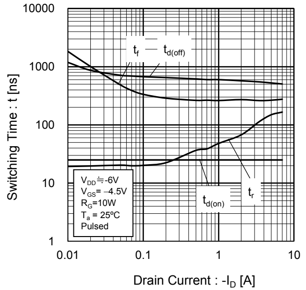
Fig.20 Switching Characteristics
