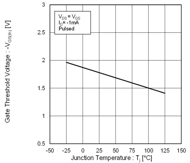
Fig.9 Gate Threshold Voltage vs. Junction Temperature
