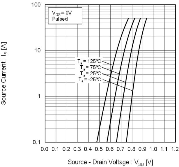
Fig.17 Source Current vs. Source Drain Voltage
