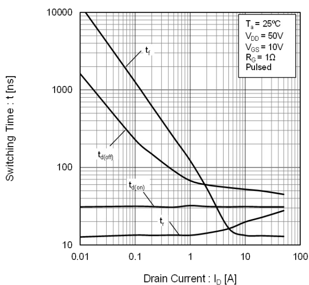
Fig.15 Switching Characteristics
