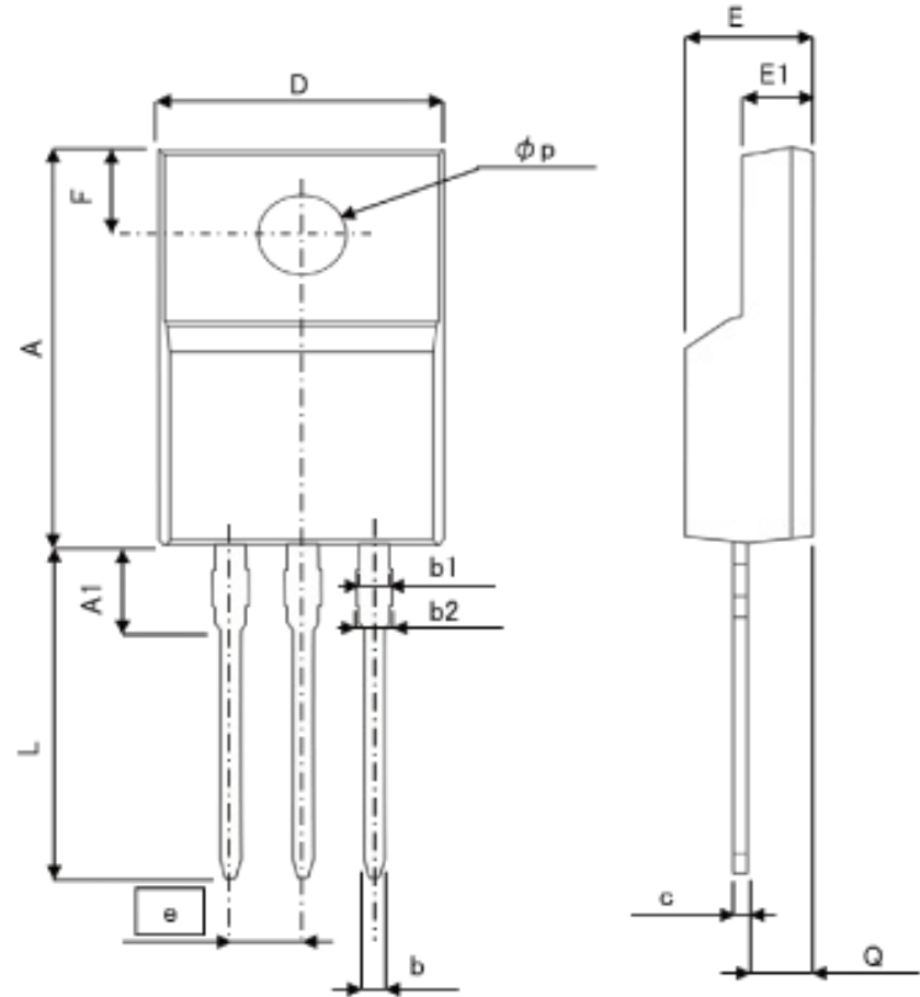
TO-220FM
