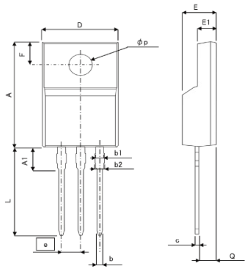
TO-220FM
