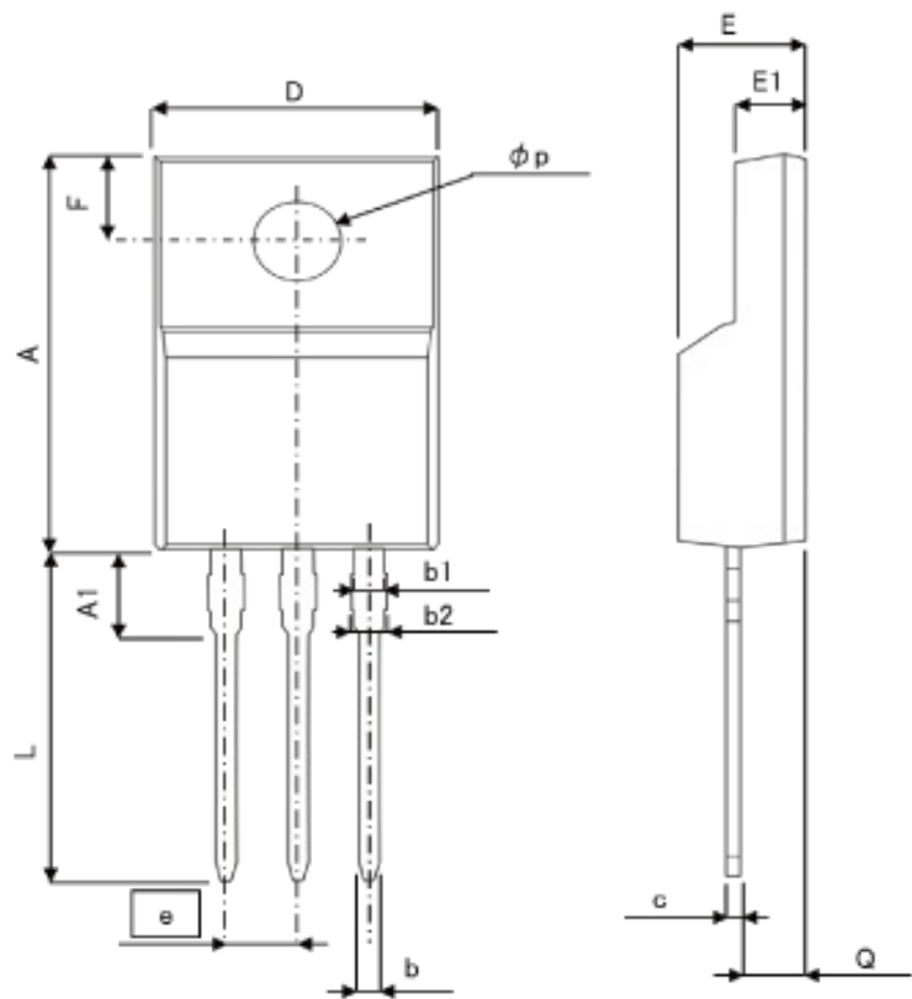
TO-220FM
