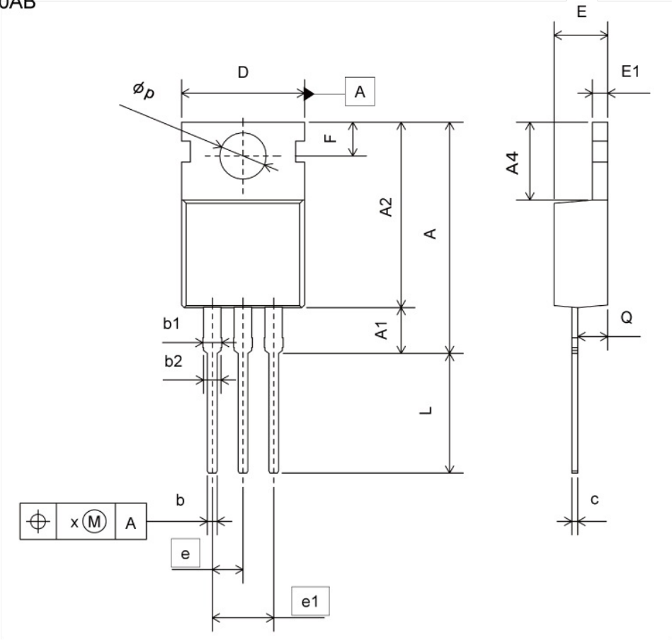
TO-220AB
