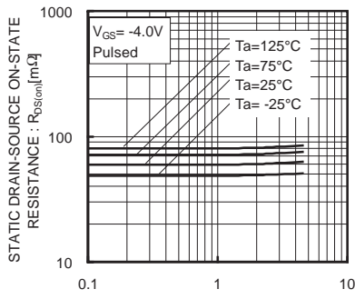
DRAIN-CURRENT : -I b [A] Fig.7 Static Drain-Source On-State Resistance vs. Drain Current (IV)
