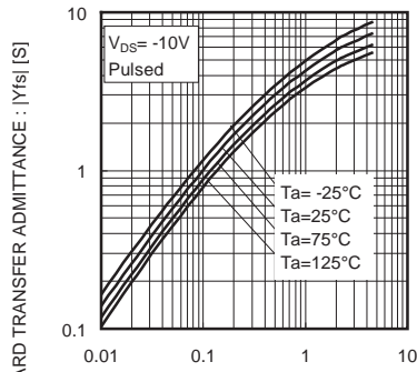
DRAIN-CURRENT : -I b [A] Fig.8 Forward Transfer Admittance vs. Drain Current
