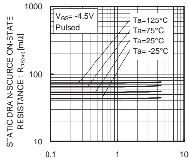
DRAIN-CURRENT : -I b [A] Fig.6 Static Drain-Source On-State Resistance vs. Drain Current (III)
