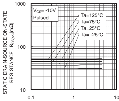
DRAIN-CURRENT : -I b [A] Fig.5 Static Drain-Source On-State Resistance vs. Drain Current (II)
