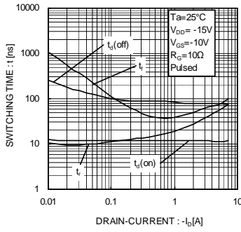
Fig.11 Switching Characteristics
