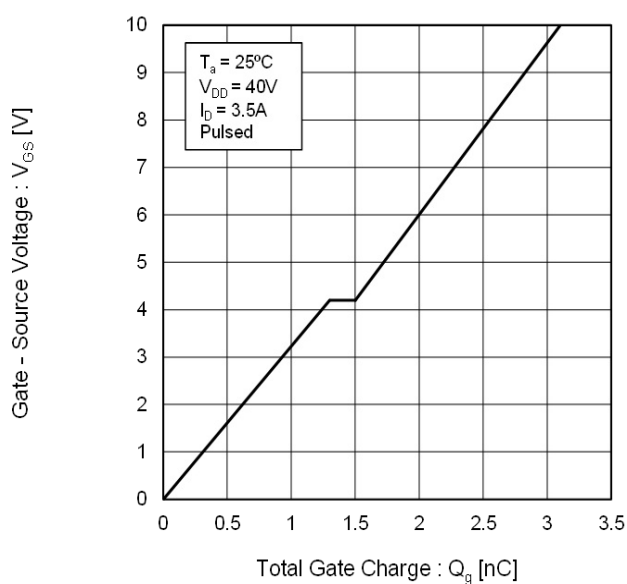
Fig.19 Typical Gate Charge
