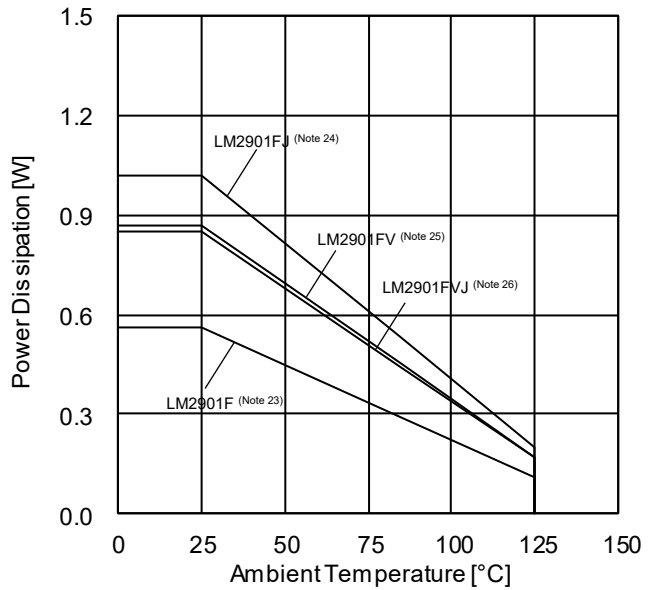
(f) LM2901xxx
