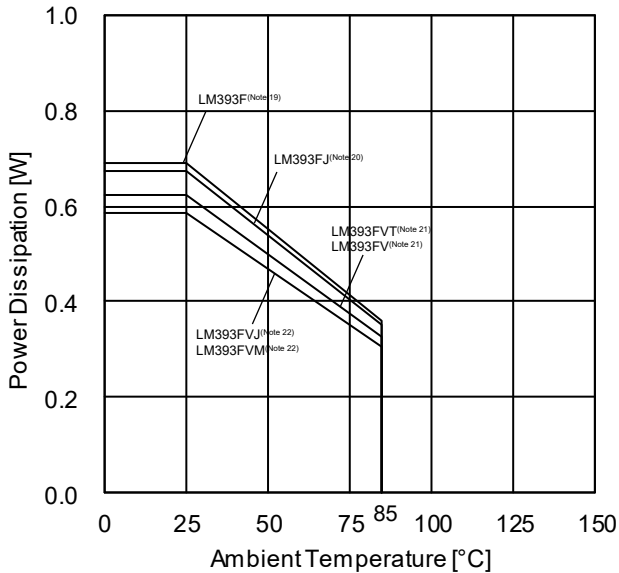
(c) LM393xxx
